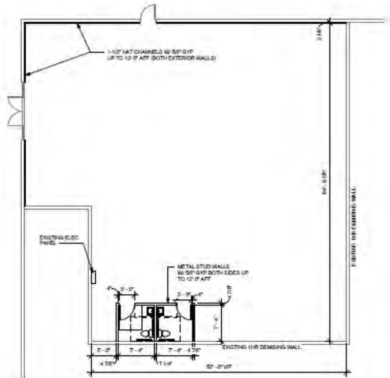
1 Floor Plan 10' x 10'
